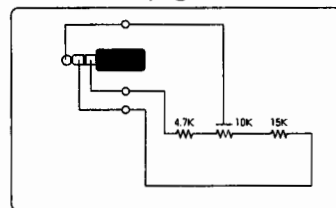
3.5mm stereo plug
